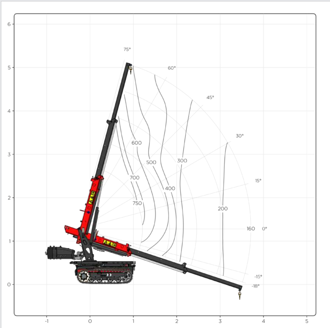
Main Boom
